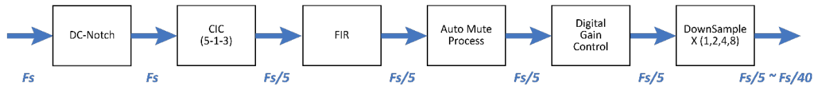
Figure 12: Digital Filter Chain
