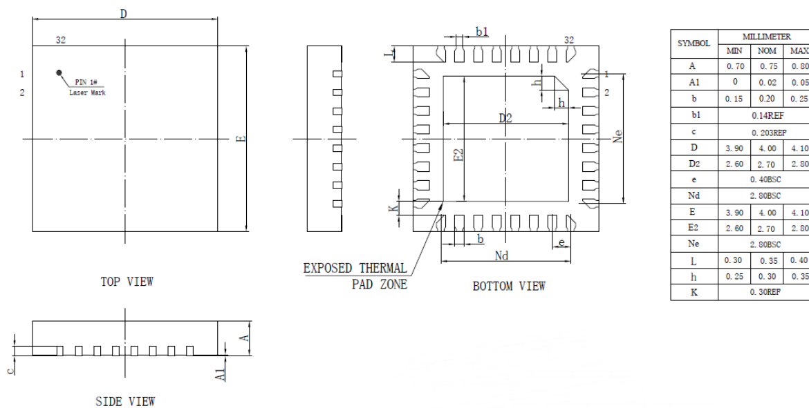
Figure 3-1 AD6976D Package
