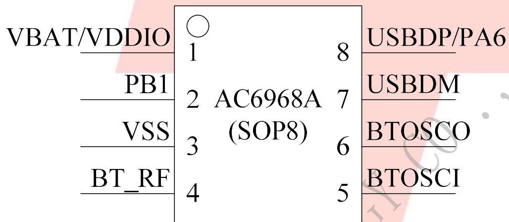
Figure 1-1 AC6968A Package Diagram
