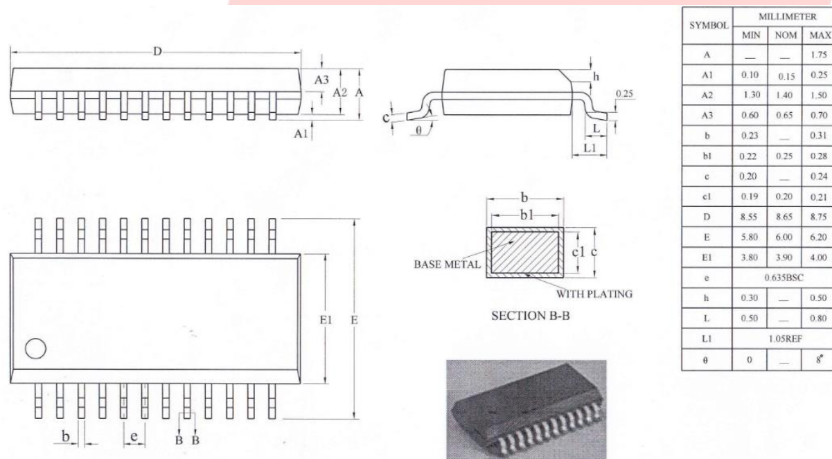
Figure 3-1. AC6965A Package
