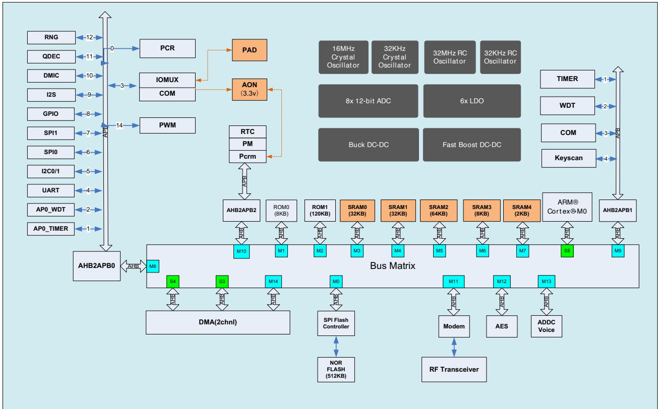
Figure 1: ST17H63 block diagram
