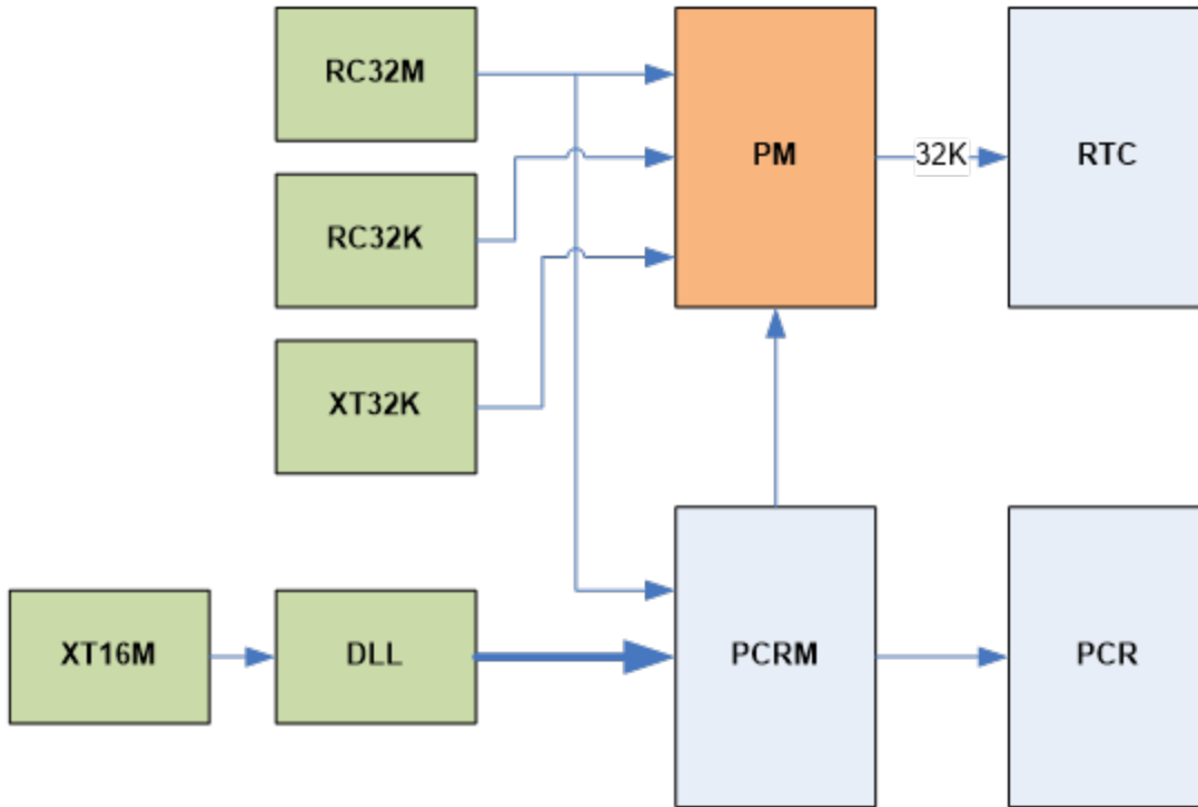
Figure 8: Clock management
