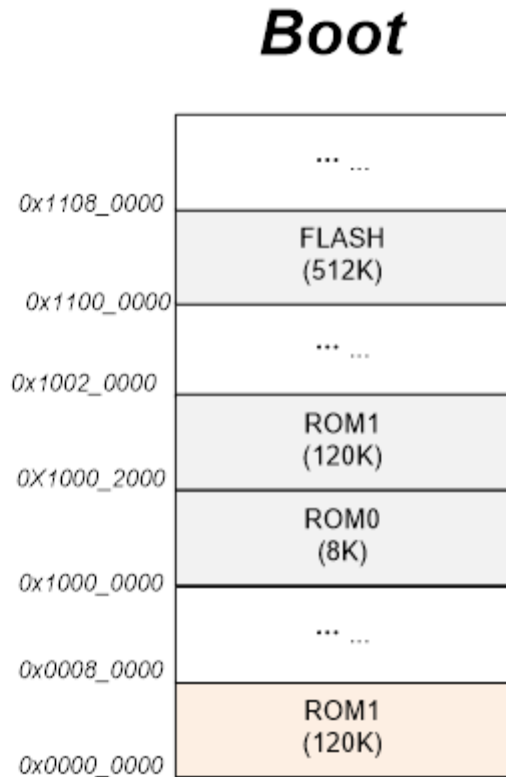
Figure 4: ST17H63 boot mode
