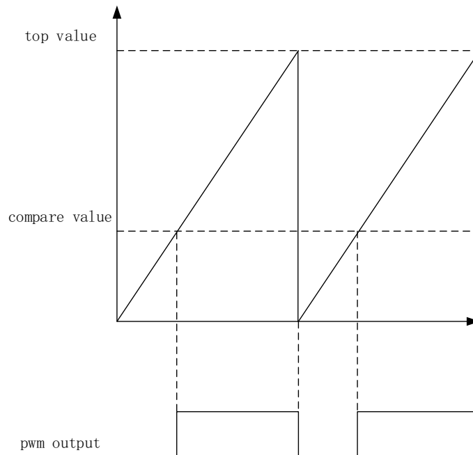
Figure 14: PWM operation
