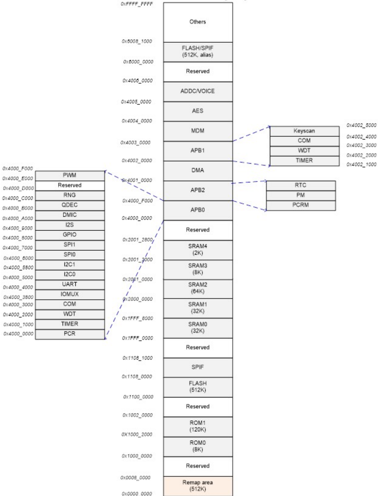
Figure 3: ST17H63 memory space
