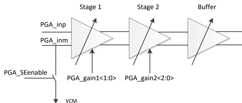
Figure 16: PGA path
