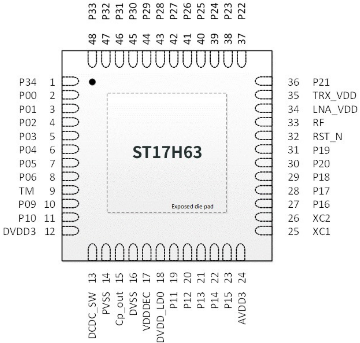
Figure 2: Pin assignment - ST17H63 QFN48 package
