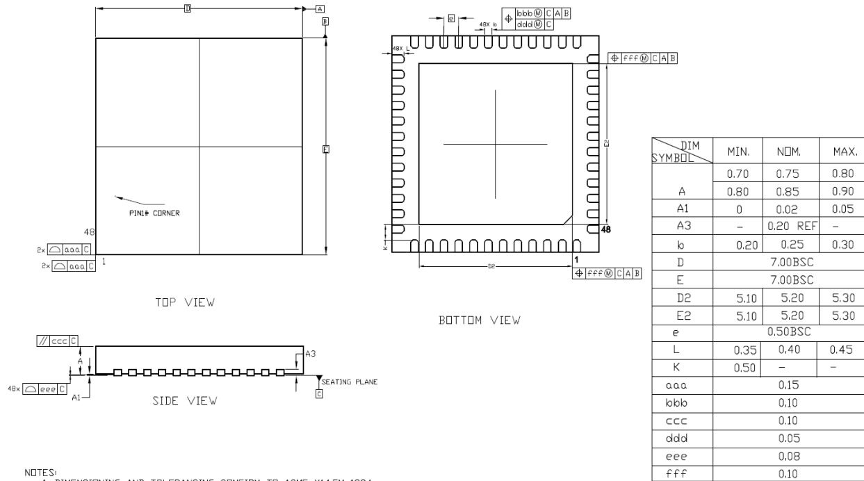
Figure 17: QFN48 package dimensions
