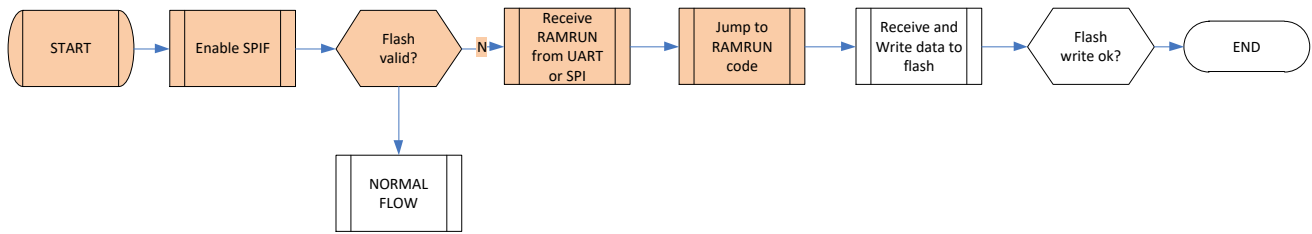
Figure 5: Bootloader flow
