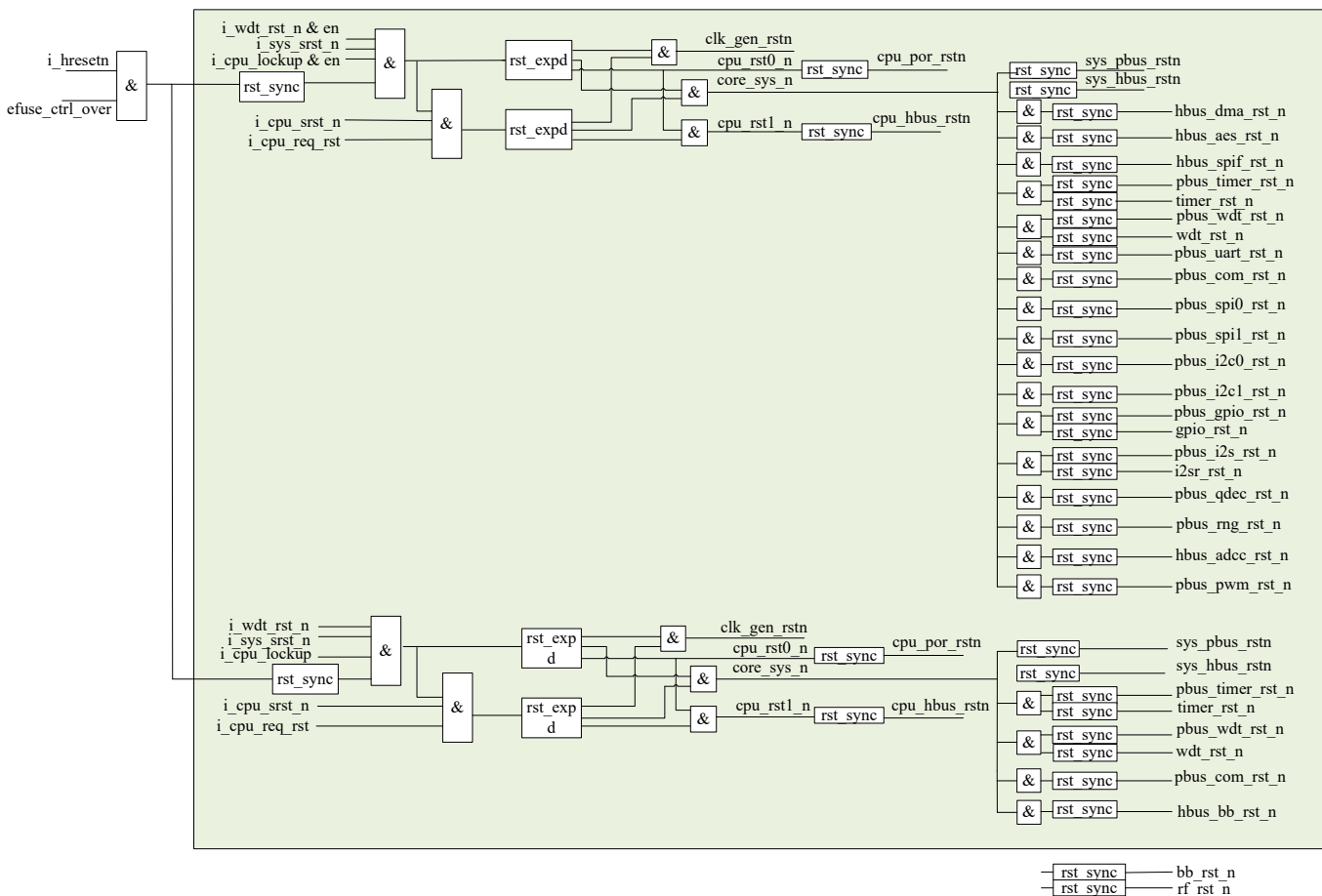
Figure 6: ST17H63 power, clock and reset
